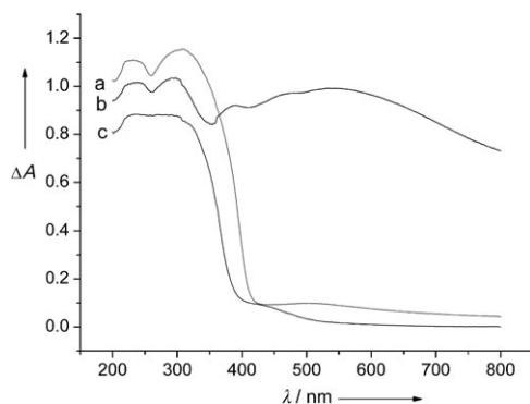
Figure 3. UV/Vis diffuse-reflectance spectra of a) AgCl, b) Ag@AgCl, and c) N-doped TiO 2 .
